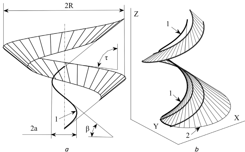
Fig. 2. Projections of the unfolded helicoid strip with the turning edge, which is helical line 1: a – frontal projection (generatrices of the unfolded helicoid are directed upwards); b – axonometric projection (generatrices of the torso-helicoid are directed downwards)
